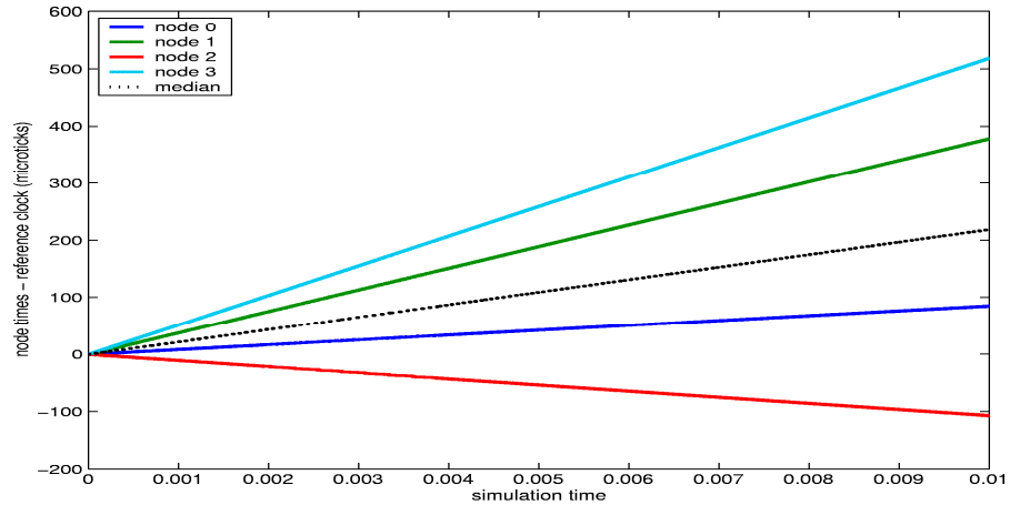
Figure 4.2: Test 1 - Free running nodes
