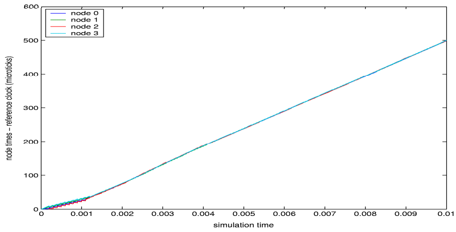
Figure 4.15: Test 6 - Cluster drift rate with rate master node 3
