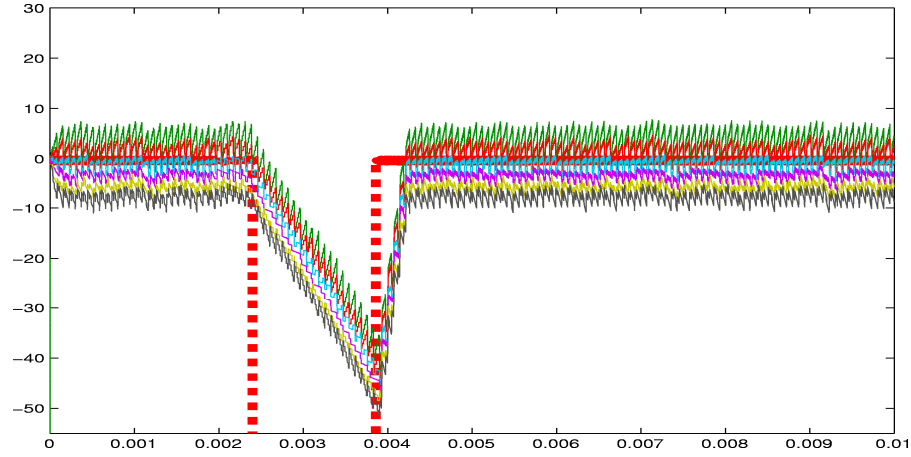
Figure 5.16: Blackout survivability - non-calibrated cluster
