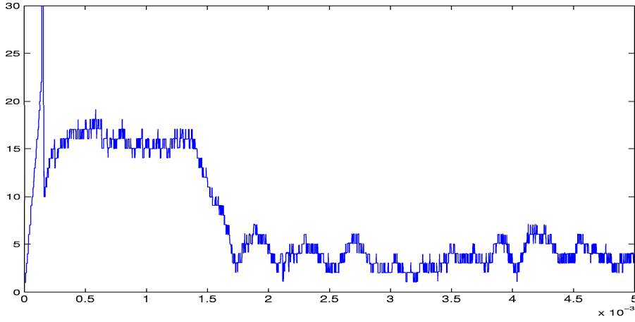
Figure 5.7: Test 2 system precision - calibrated clusters
