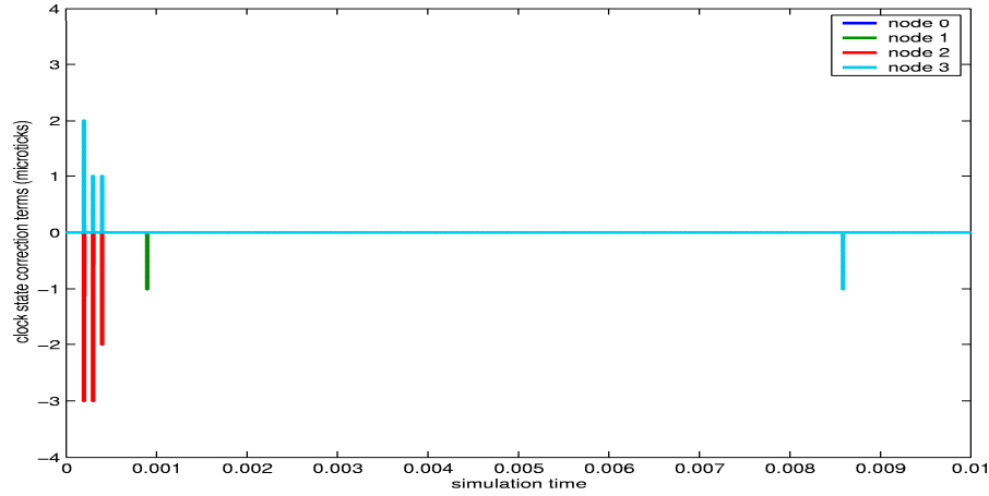
Figure 4.7: Test 4 - Clock state correction terms
