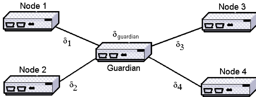
Figure 3.6: Transmission delay - star topology
