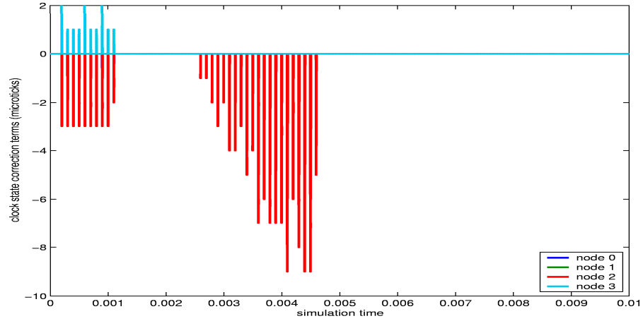
Figure 4.10: Test 5 - Clock state correction terms
