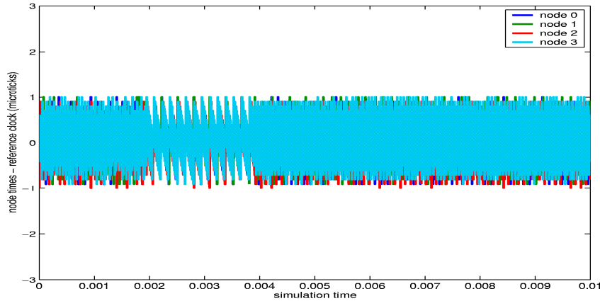
Figure 4.3: Test 2 - Free running nodes
