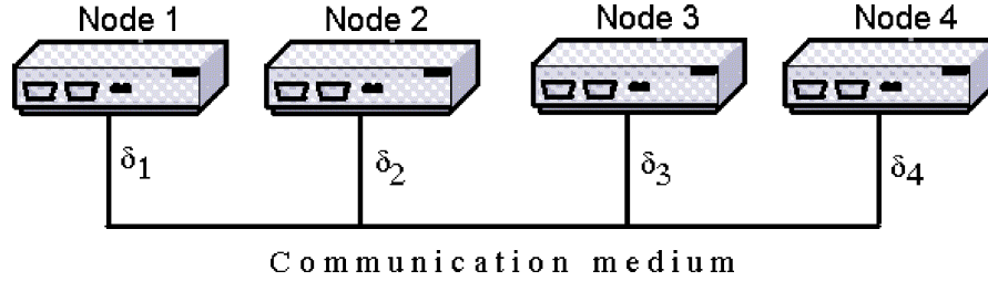
Figure 3.5: Transmission delay - bus topology
