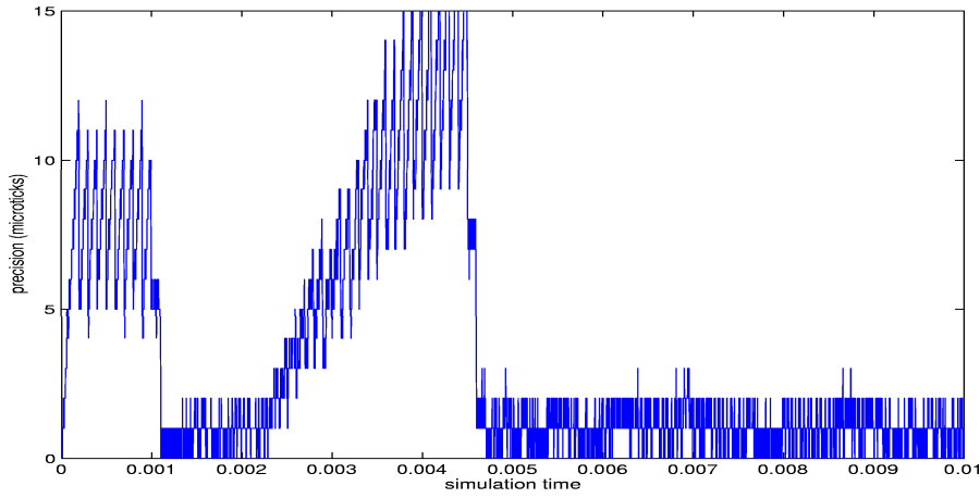
Figure 4.8: Test 5 - Cluster precision
