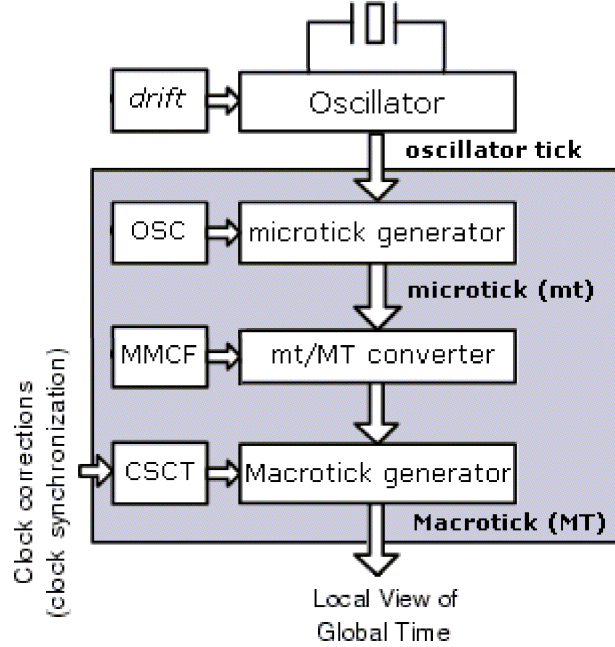
Figure 3.2: Local time
