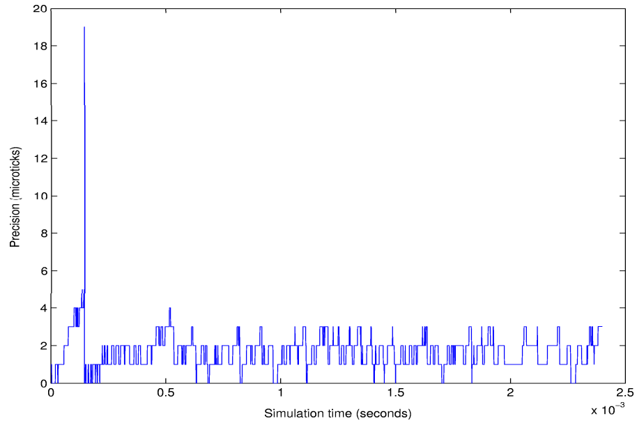
Figure C.3: Reference Test 5 - Cluster precision
