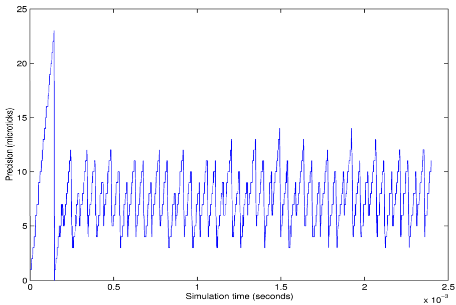
Figure C.1: Reference Test 2 - Cluster precision
