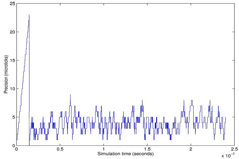
Figure C.2: Reference Test 3 - Cluster precision
