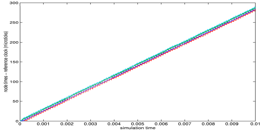
Figure 4.5: Test 3 - Cluster drift rate
